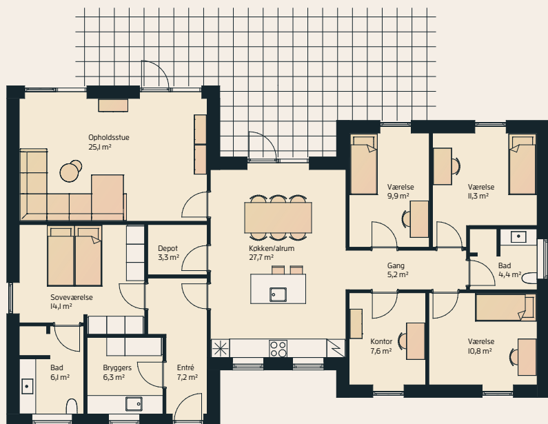
H-hus 169 m²
