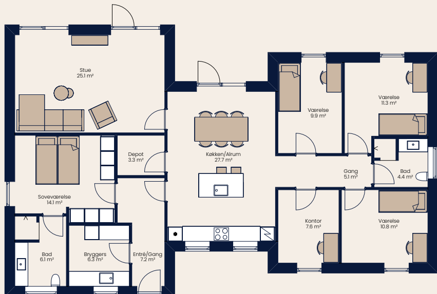
H-hus 169 m 2
